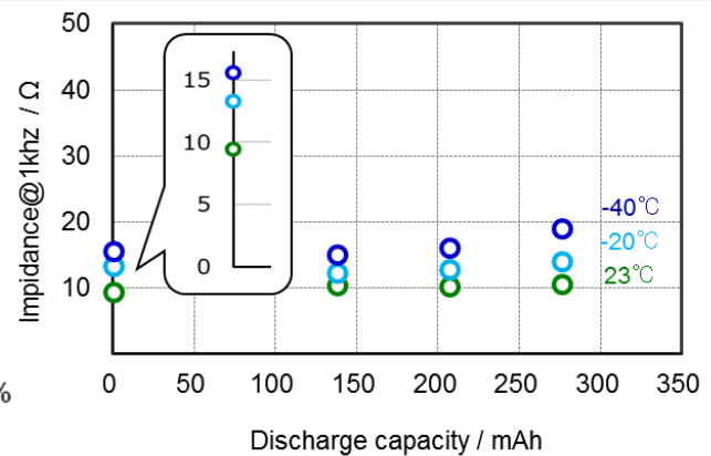
Impedance by Temperature
