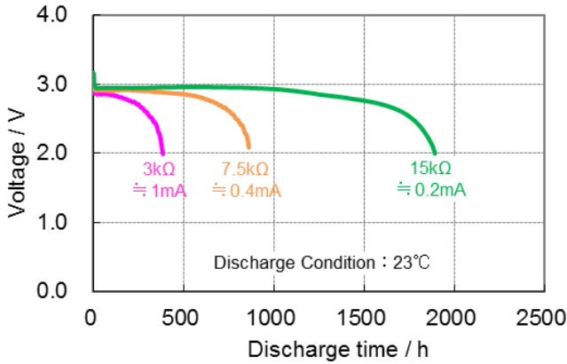
Discharge Characteristics by Load
