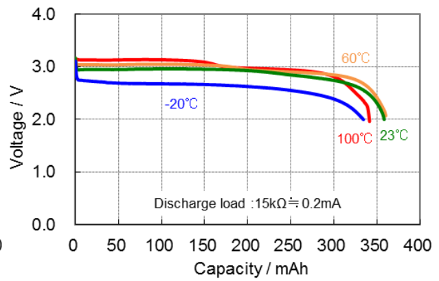
Discharge Characteristics by Temperature
