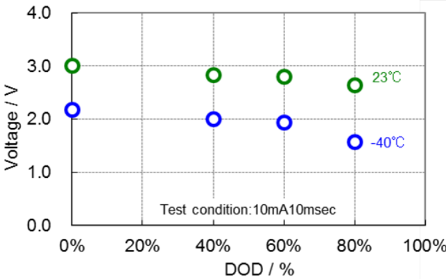
Closed Circuit Voltage by Temperature
